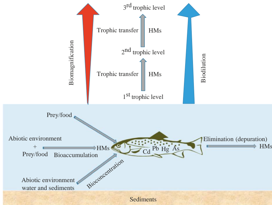
FIGURE 3: Schematic summarizing terms and concepts involved in trophodynamics of heavy metals ([62], used with permission of Tailor and Francis).
